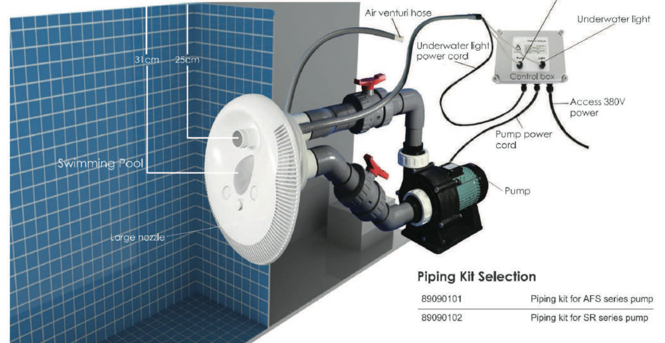
Counter Current Jet System Installation (with 1 pump setting)
